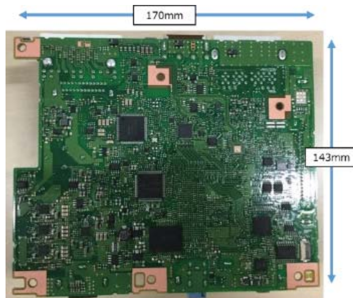
Component Side(Cockpit Control Unit) – Main PCB
