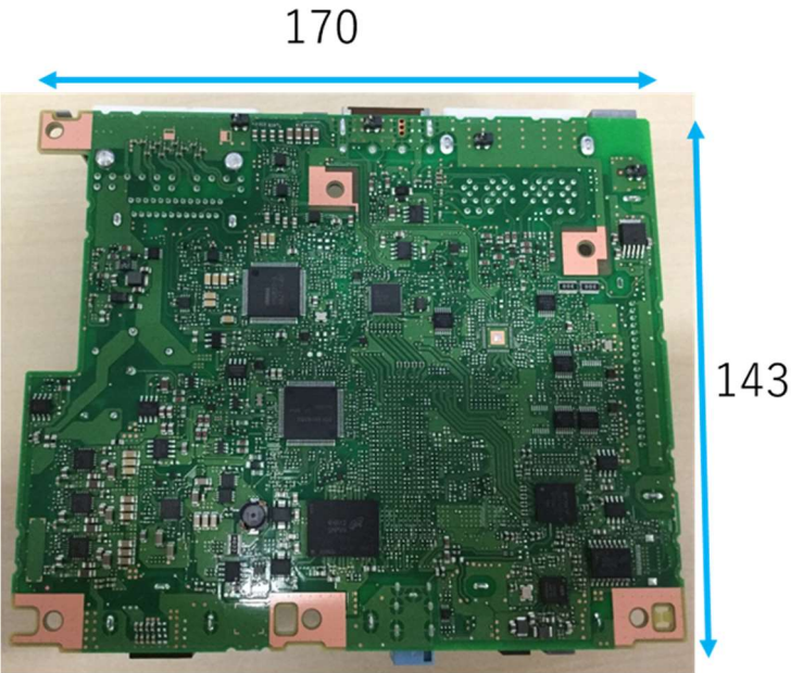
Component Side (Main PCB)
