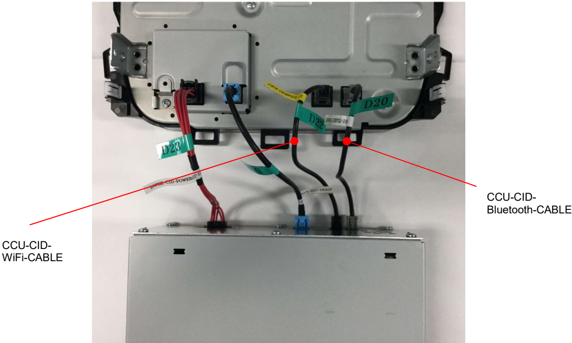
Connection parts of the CCU and CID
