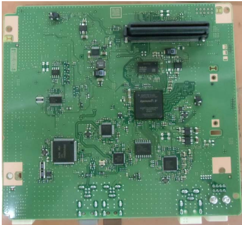
Solder Side(Main PCB)
