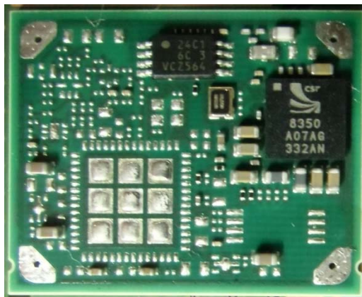
Top (without a cover)
