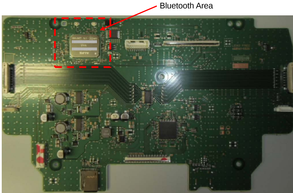
(Component Side)
