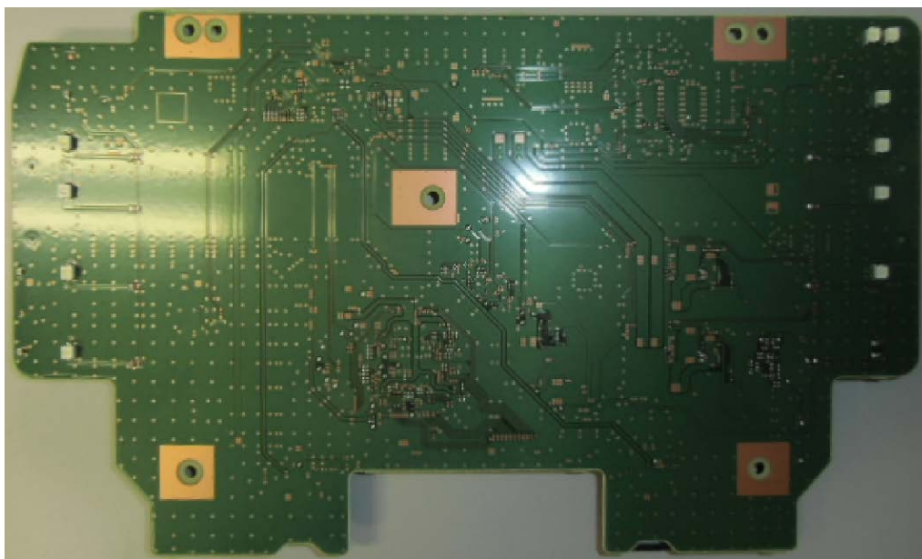
(Solder Side)
