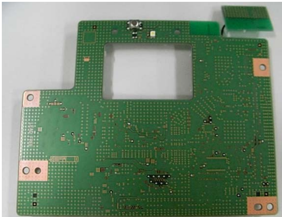
PCB including Bluetooth IC (Solder Side)
