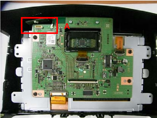
Back view
