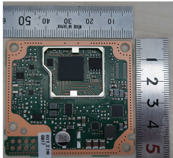
Component side (Without Shield)
