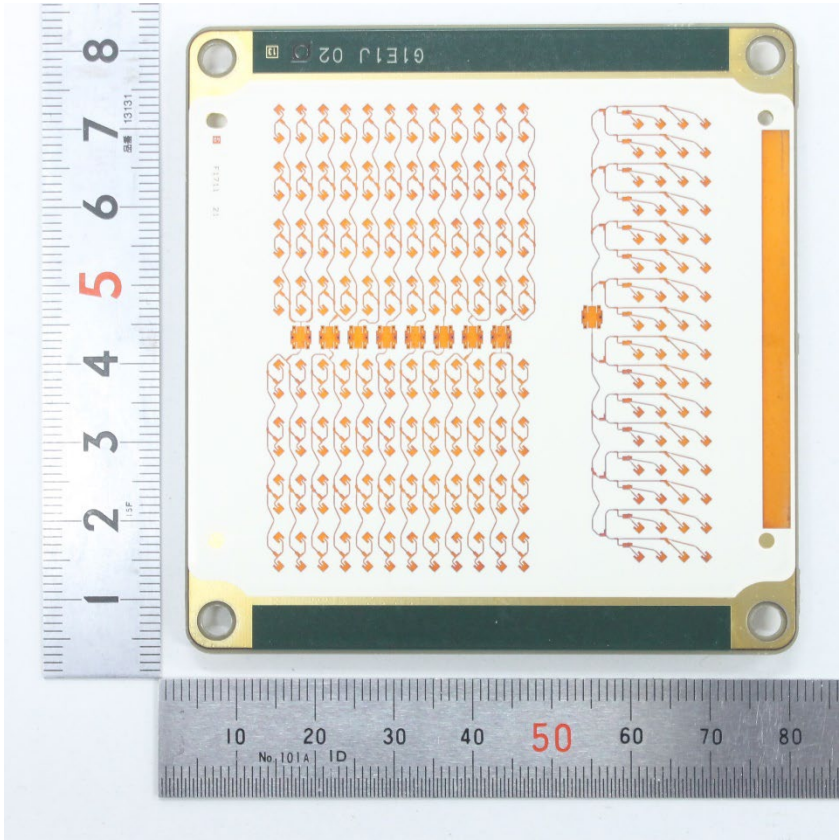
Antenna side
