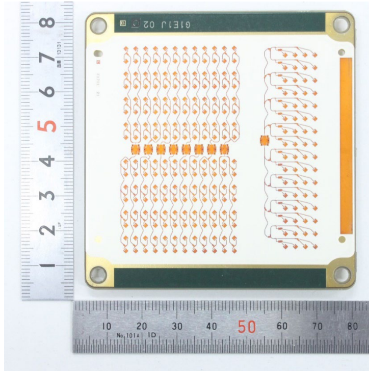
Antenna side
