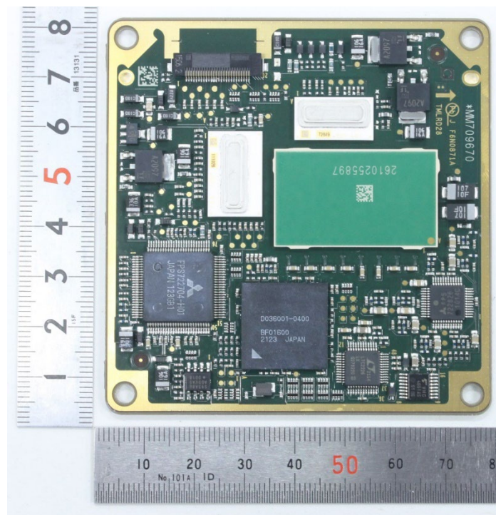
Component side
