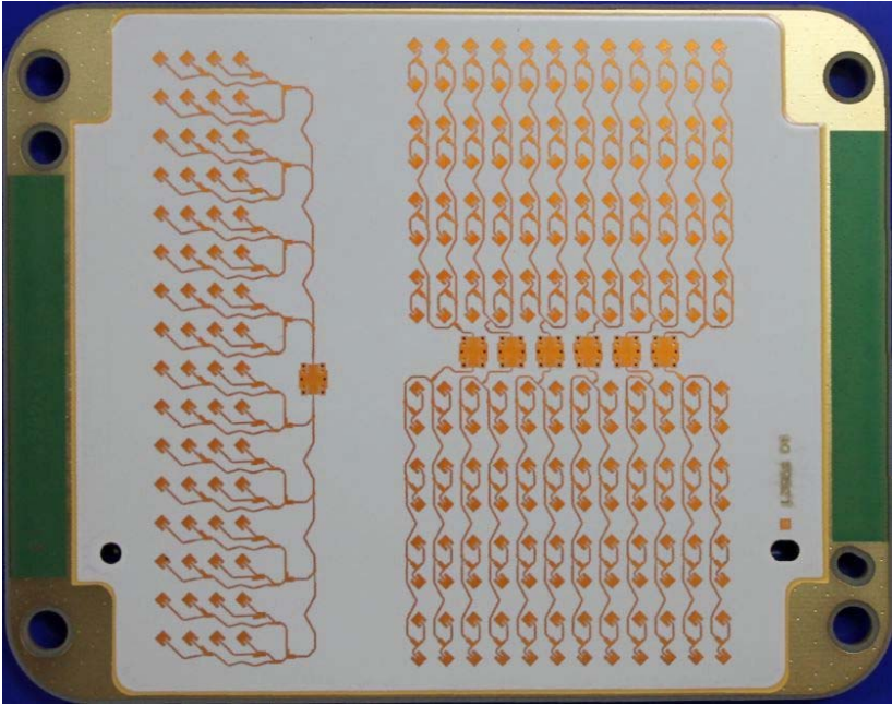
Antenna side
