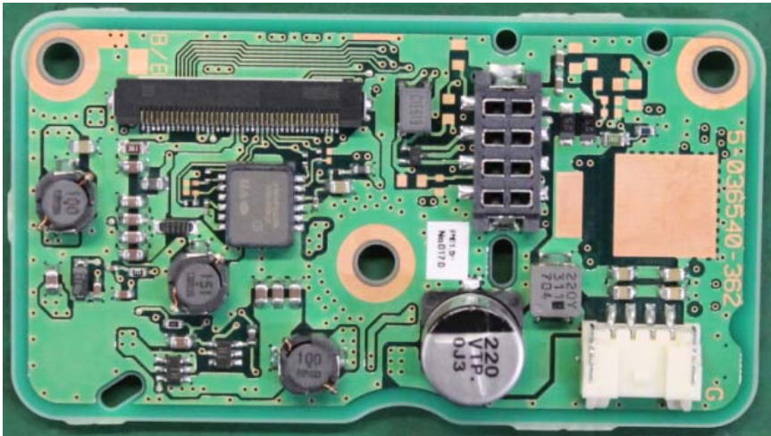
Component side B
