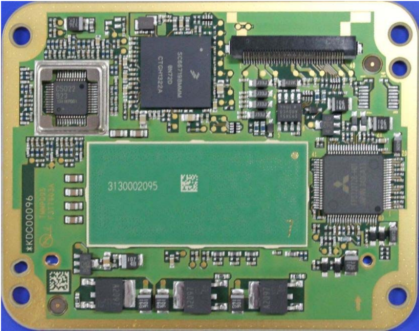
Component side
