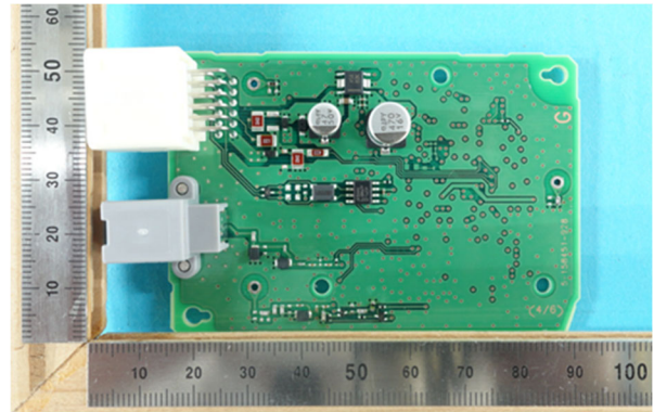
Component side without antenna
