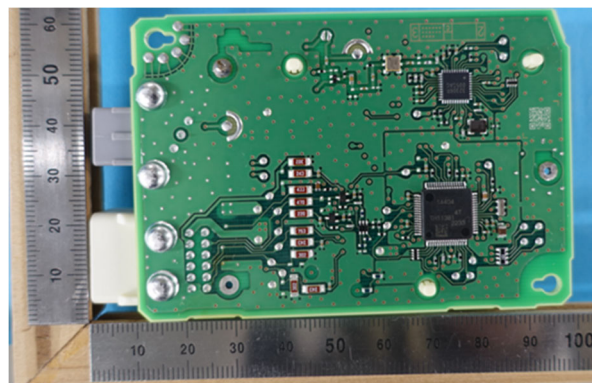
Solder side
