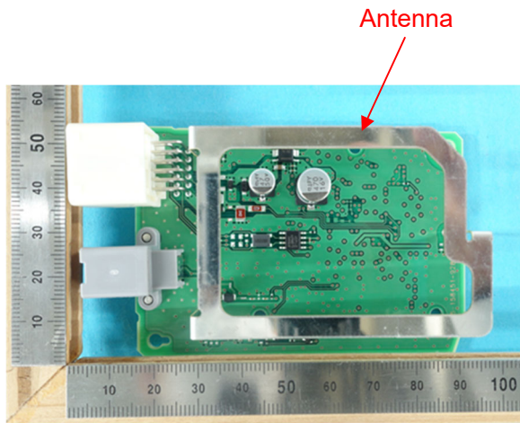
Component side with antenna
