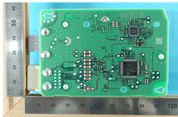
Solder side
