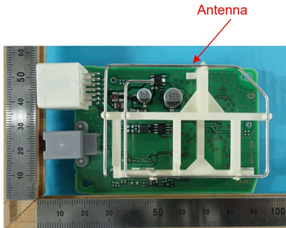
Component side with antenna
