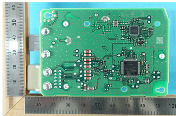
Solder side
