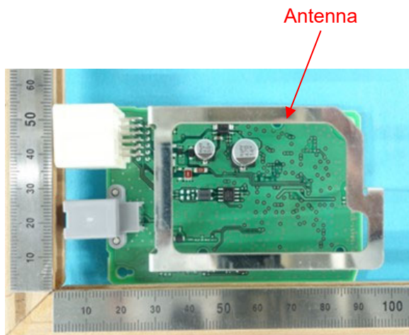
Component side with antenna
