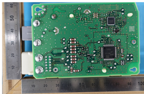
Solder side
