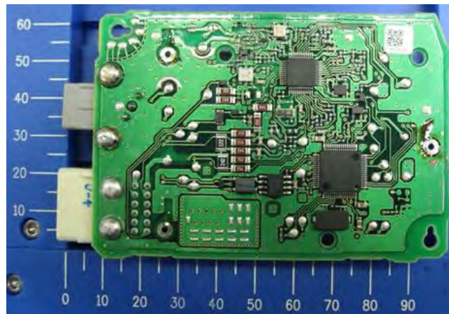
Solder Side
