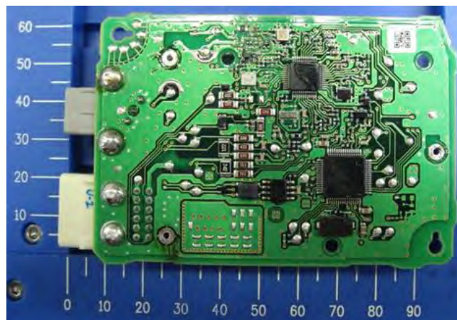
Solder Side
