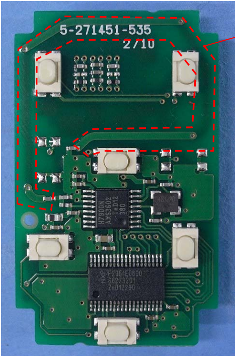
Comp. Side
