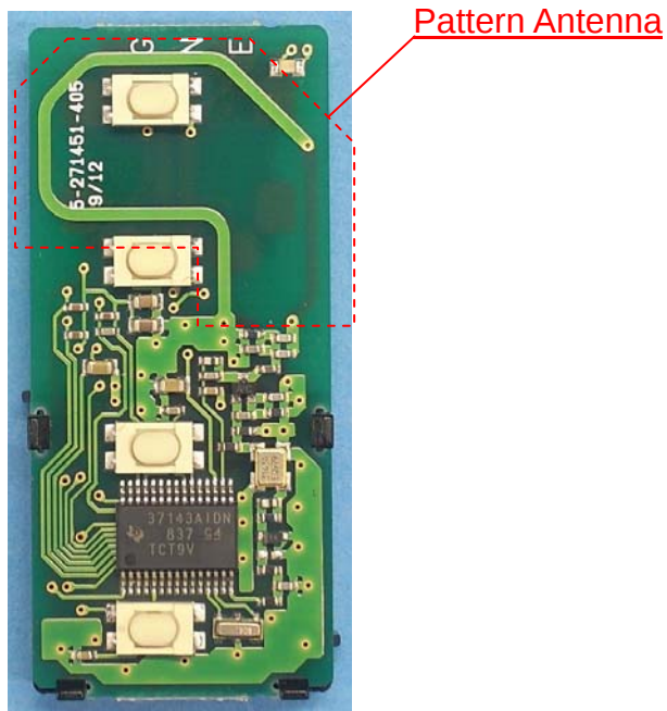
Comp. Side
