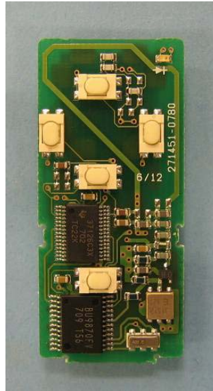
Comp Side
