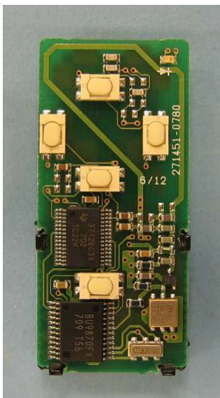
Comp Side
