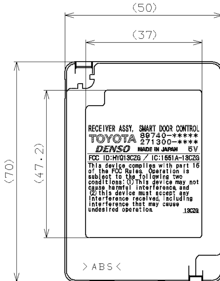
Fig. Marking location and layout of Receiver
