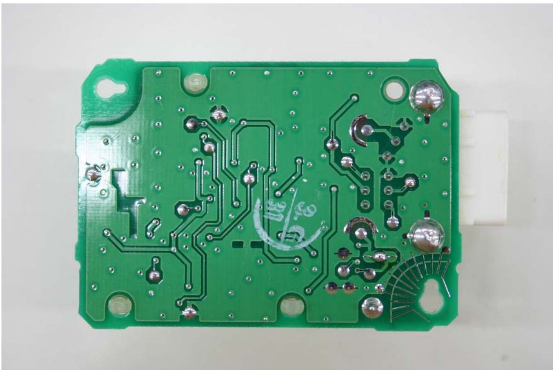
Solder side
