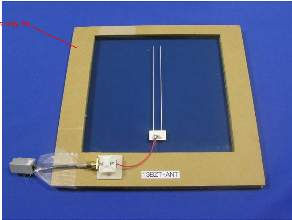
Printed Antenna on the glass (front)
