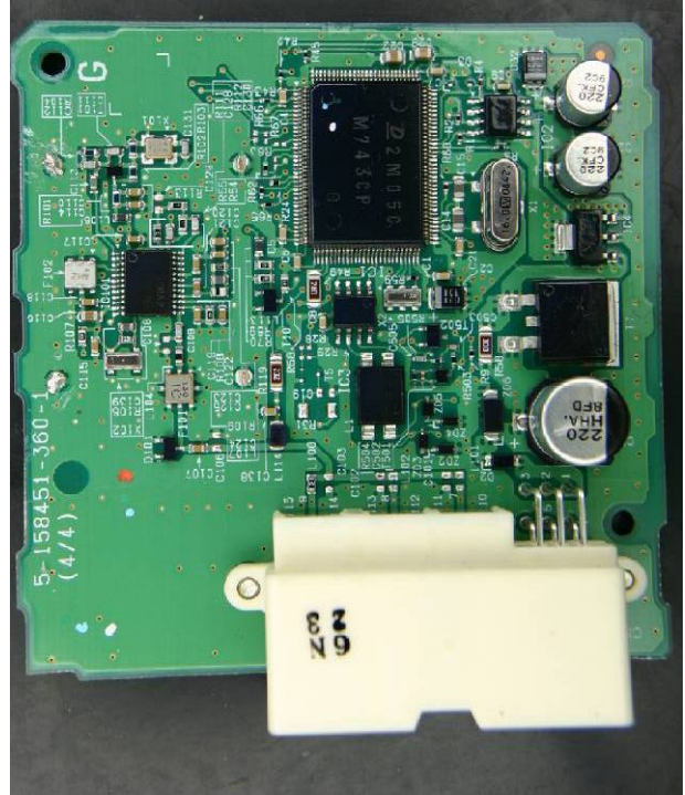
Comp Side
