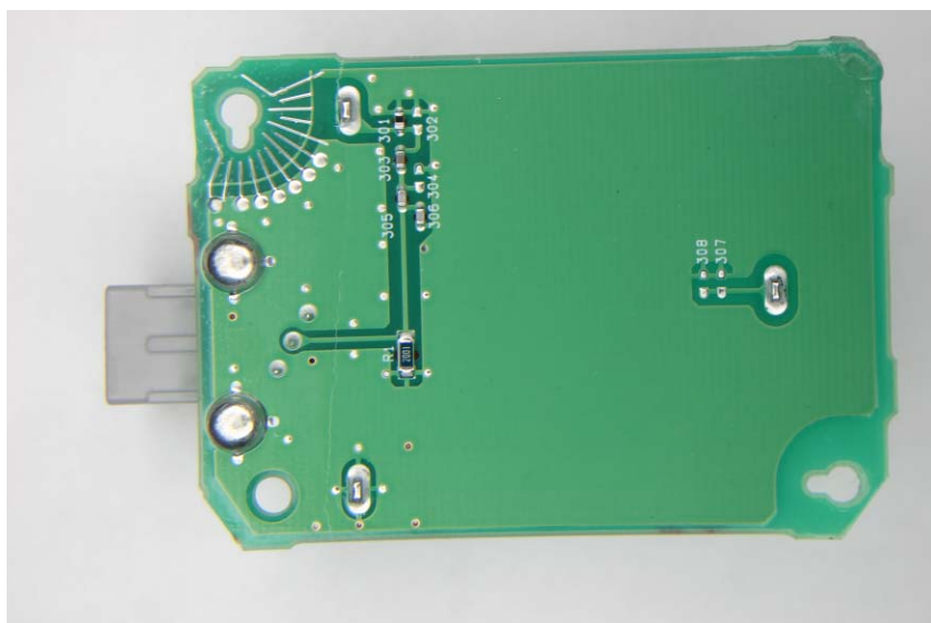
Solder Side
