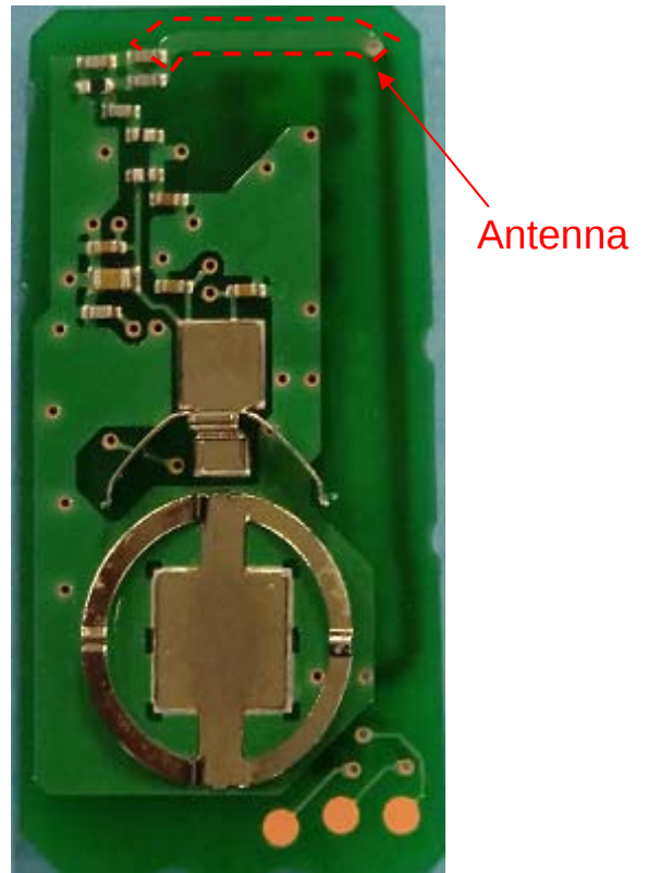
Solder Side
