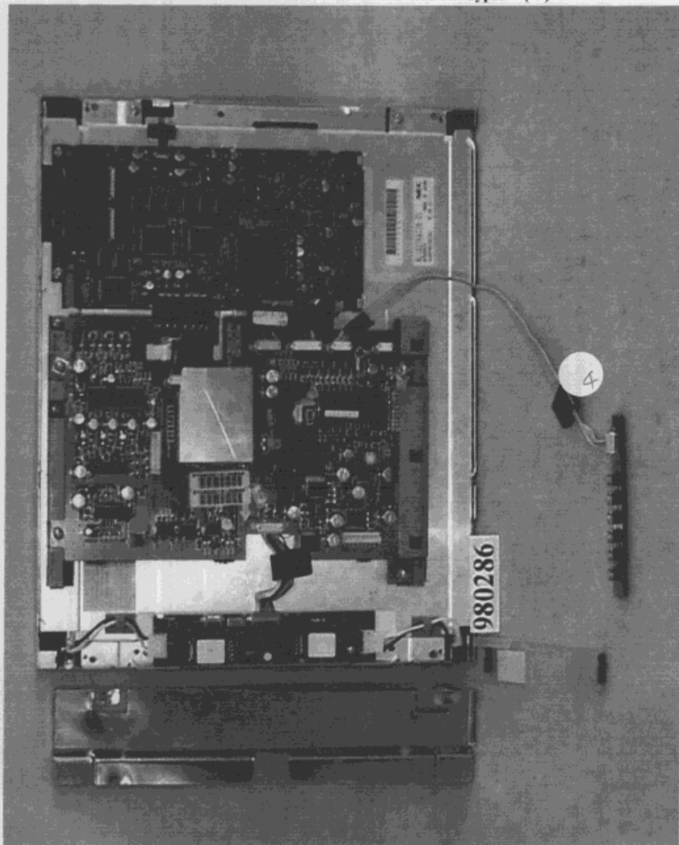
The Rear View of LCD Panel with a ferrite core on keypad - ( 4 )
