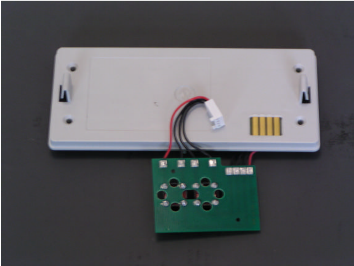
FILTER FOIL
