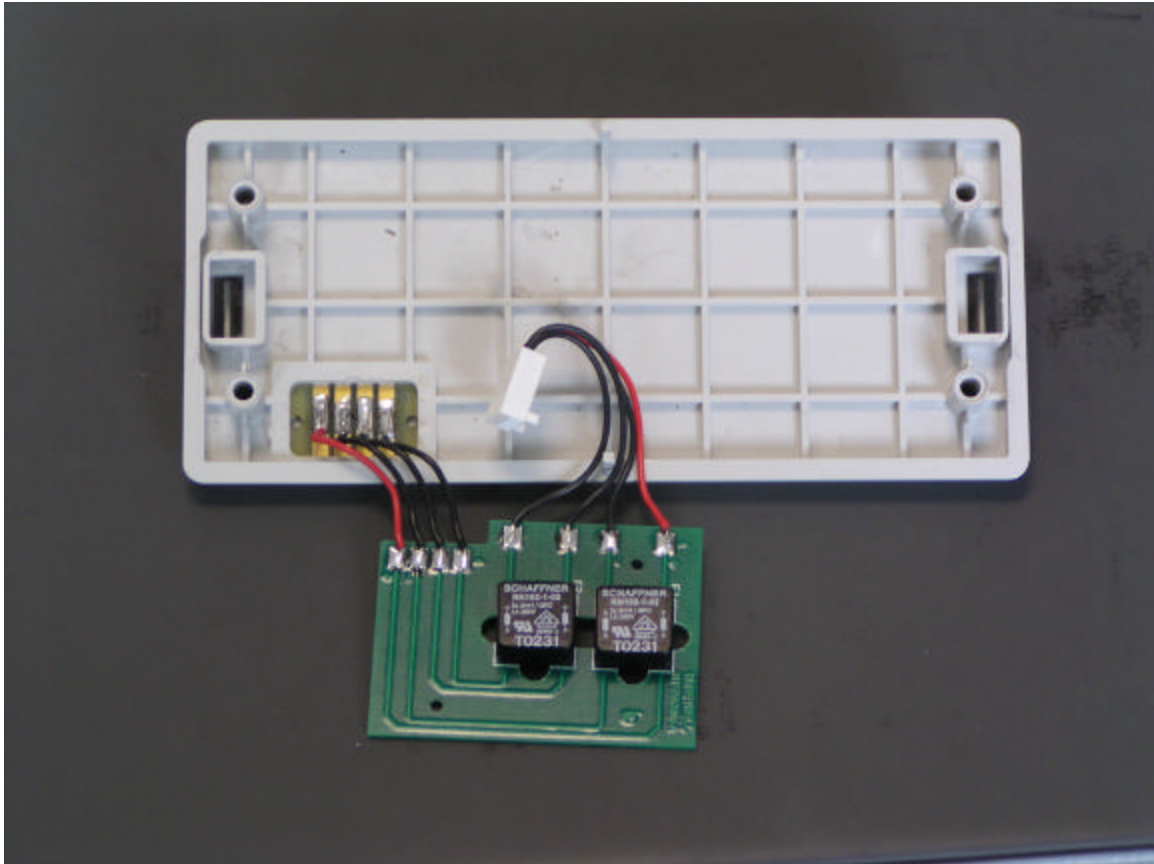
FILTER COMPONENTS
