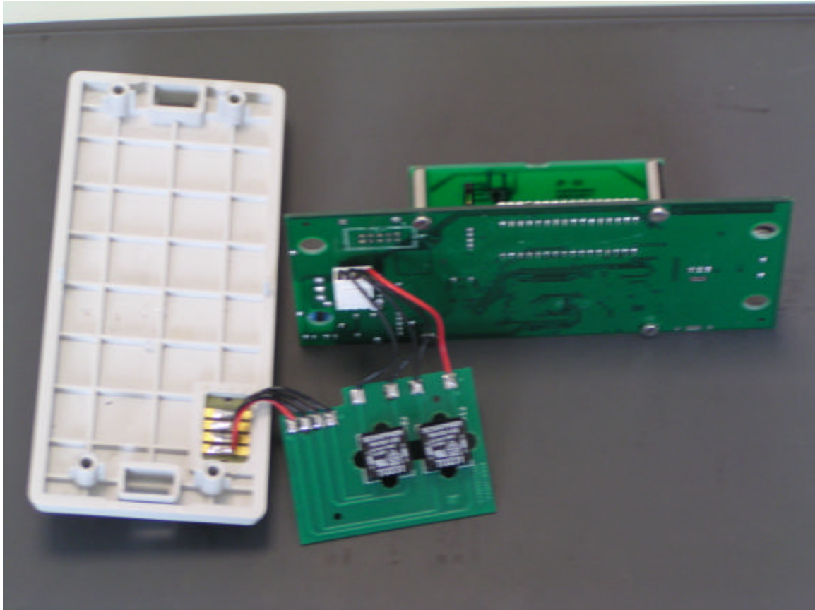
PARTIAL DISASSEMBLED
