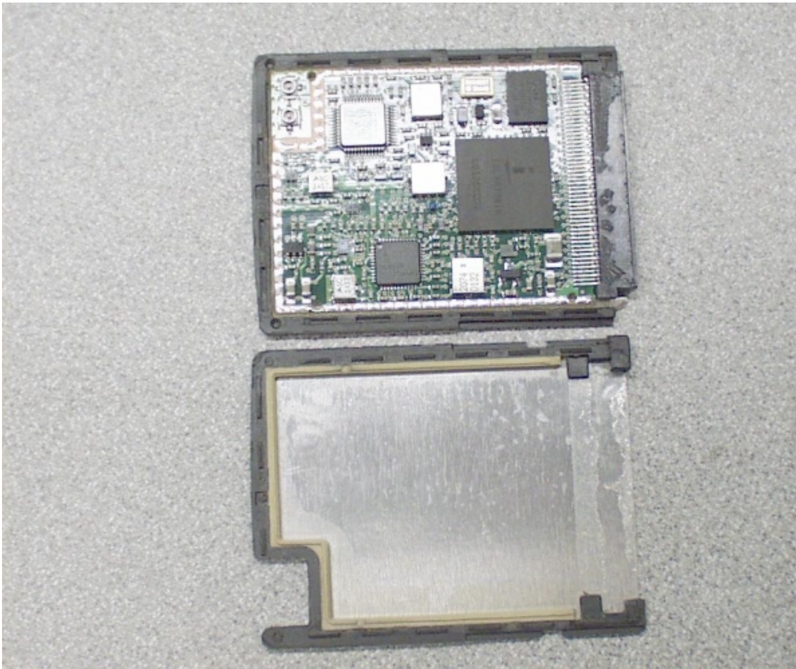
Top of Radio, Shield Removed
