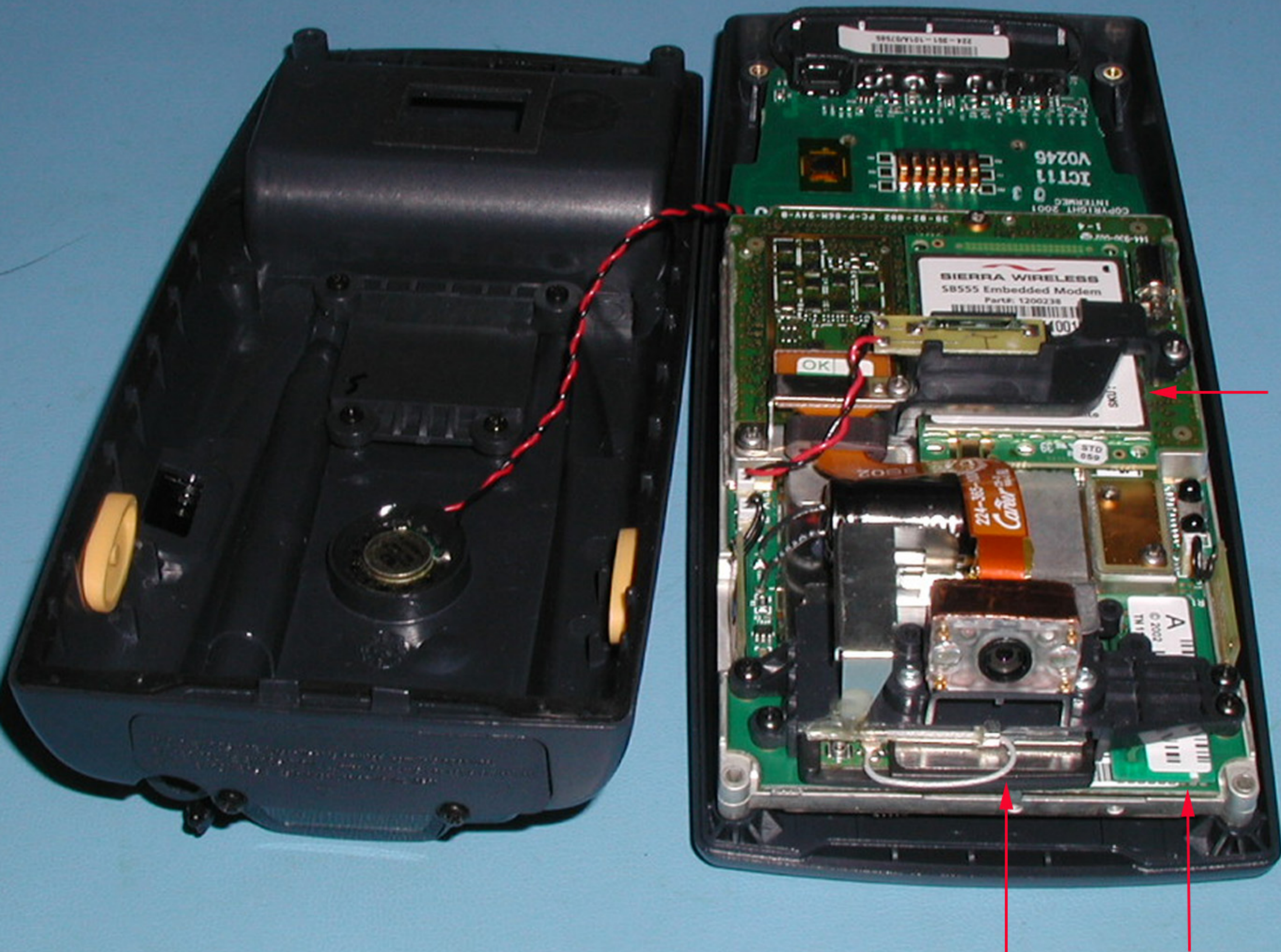
CDMA, 802.11b & Bluetooth Radios Configuration
