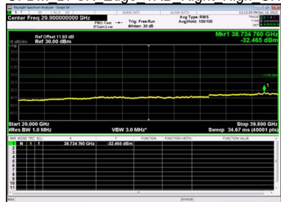
N77(100M)_DFT-s- OFDM BPSK Edge 1RB Right High CH
