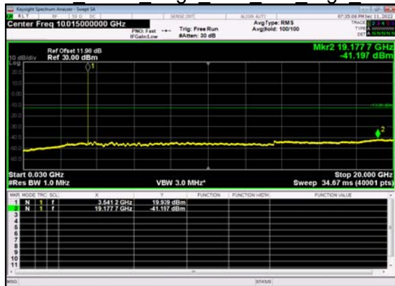
N77(10M)_DFT-s- OFDM BPSK Edge 1RB Left High CH
