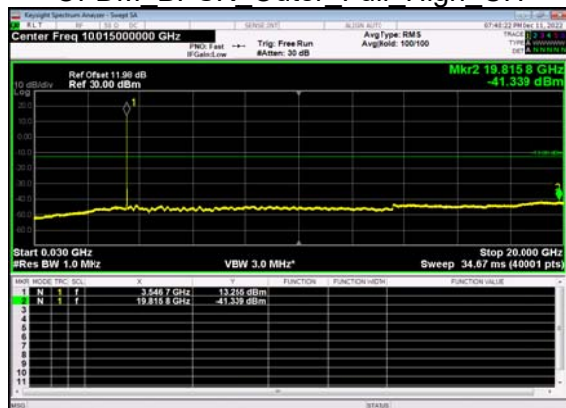
N77(10M)_DFT-s- OFDM BPSK Outer Full High CH
