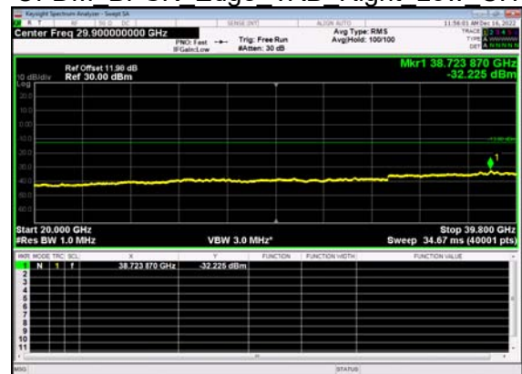
N77(100M)_DFT-s- OFDM BPSK Edge 1RB Right Low CH
