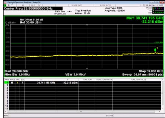
N77(100M)_DFT-s- OFDM QPSK Edge 1RB Right Low CH
