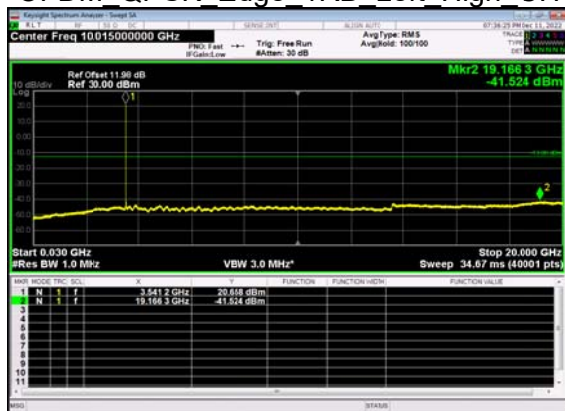
N77(10M)_DFT-s- OFDM QPSK Edge 1RB Left High CH
