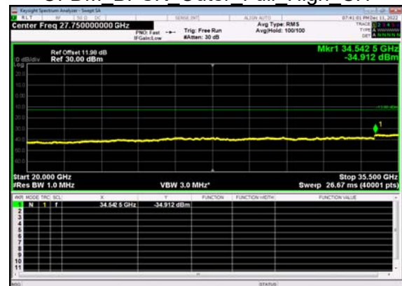
N77(10M)_DFT-s- OFDM BPSK Outer Full High CH
