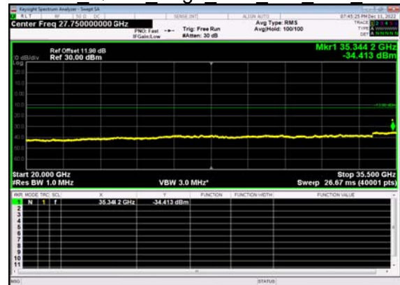
N77(15M)_DFT-s- OFDM QPSK Edge 1RB Left Low CH
