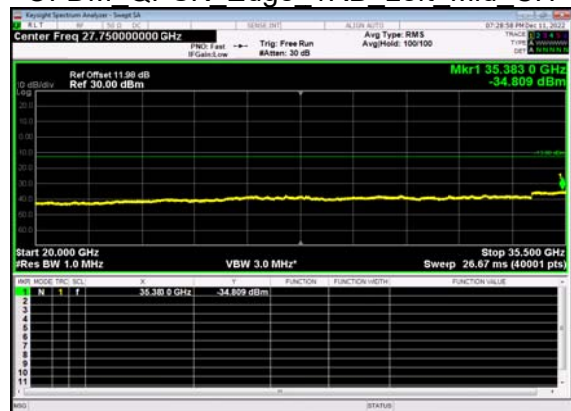
N77(10M)_DFT-s- OFDM QPSK Edge 1RB Left Mid CH
