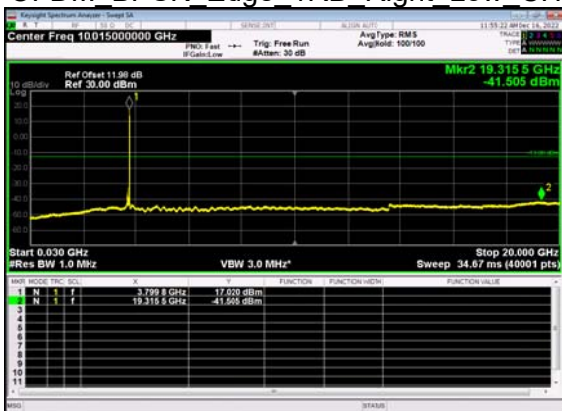
N77(100M)_DFT-s- OFDM BPSK Edge 1RB Right Low CH
