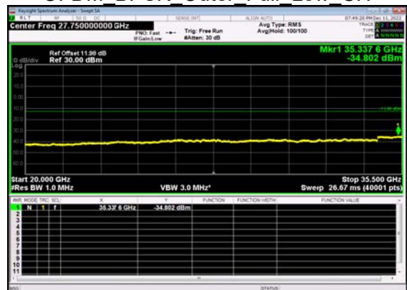
N77(15M)_DFT-s- OFDM BPSK Outer Full Low CH
