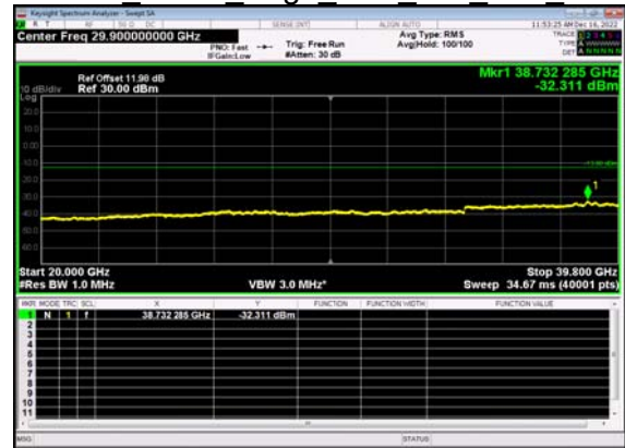
N77(100M)_DFT-s- OFDM BPSK Edge 1RB Left Low CH
