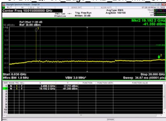
N77(10M)_DFT-s- OFDM QPSK Edge 1RB Left Mid CH
