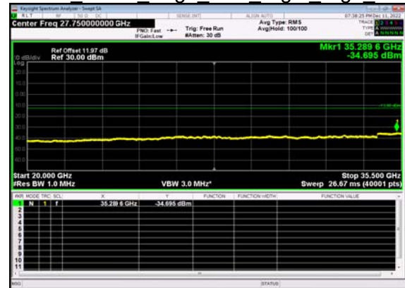
N77(10M)_DFT-s- OFDM BPSK Edge 1RB Right High CH
