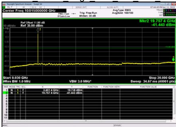
N77(15M)_DFT-s- OFDM QPSK Edge 1RB Left Low CH
