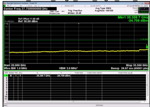
N77(10M)_DFT-s- OFDM BPSK Edge 1RB Right Low CH
