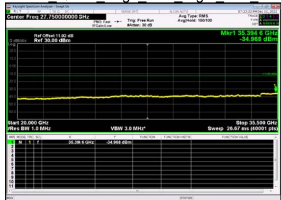
N77(10M)_DFT-s- OFDM QPSK Edge 1RB Right Low CH
