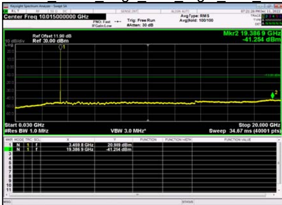
N77(10M)_DFT-s- OFDM BPSK Edge 1RB Right Low CH
