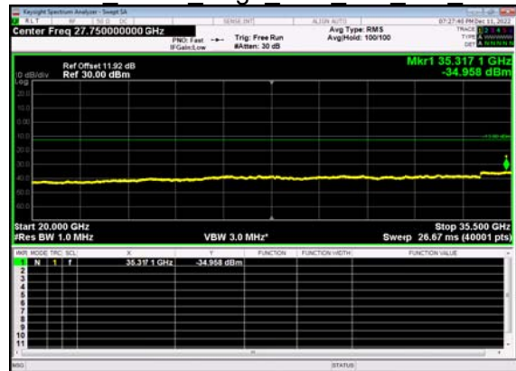
N77(10M)_DFT-s- OFDM BPSK Edge 1RB Left Mid CH
