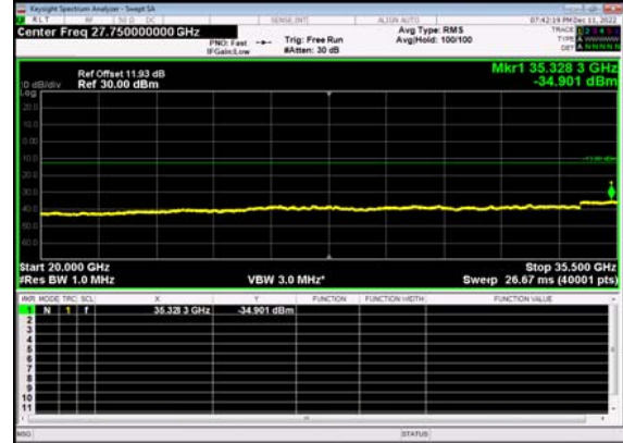
N77(10M)_DFT-s- OFDM QPSK Outer Full High CH
