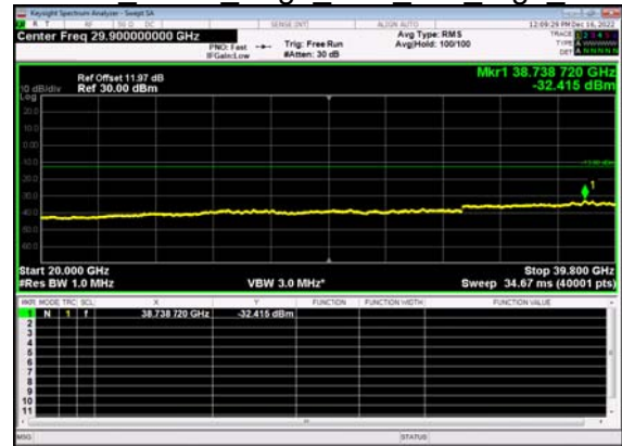
N77(100M)_DFT-s- OFDM BPSK Edge 1RB Left High CH
