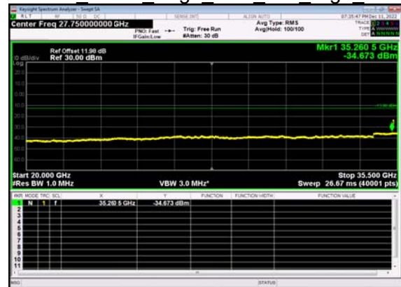
N77(10M)_DFT-s- OFDM BPSK Edge 1RB Left High CH
