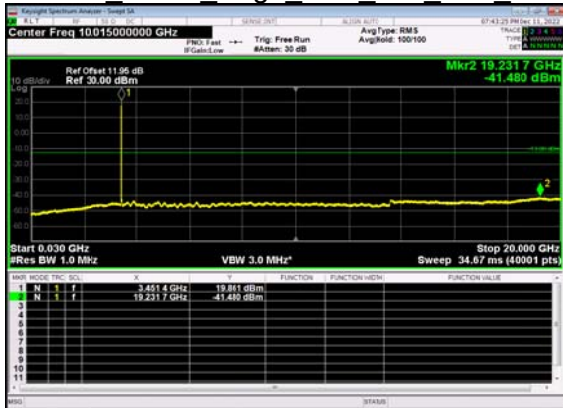
N77(15M)_DFT-s- OFDM BPSK Edge 1RB Left Low CH
