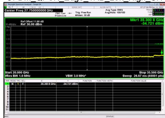
N77(10M)_DFT-s- OFDM QPSK Edge 1RB Left High CH
