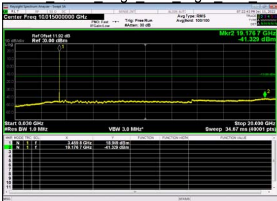
N77(10M)_DFT-s- OFDM QPSK Edge 1RB Right Low CH
