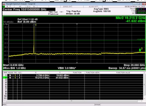
N77(60M)_DFT-s- OFDM BPSK Edge 1RB Right Low CH
