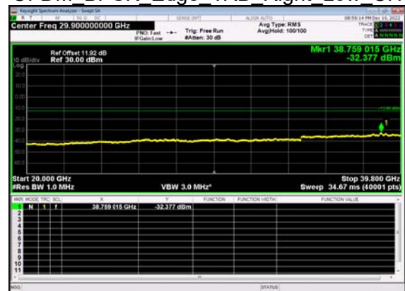
N77(60M)_DFT-s- OFDM BPSK Edge 1RB Right Low CH
