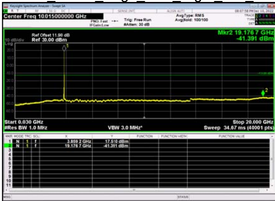
N77(40M)_DFT-s- OFDM QPSK Edge 1RB Right Mid CH
