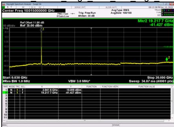
N77(40M)_DFT-s- OFDM QPSK Edge 1RB Left High CH
