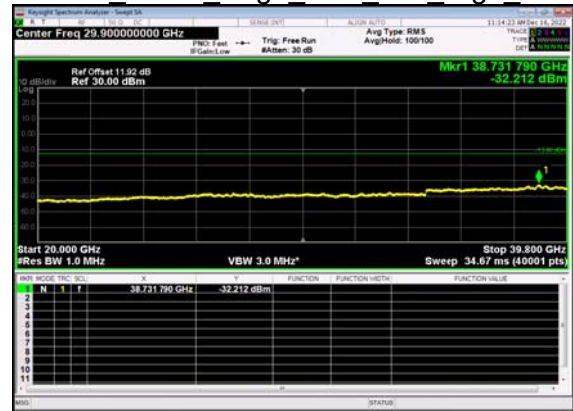
N77(80M)_DFT-s- OFDM BPSK Edge 1RB Left High CH
