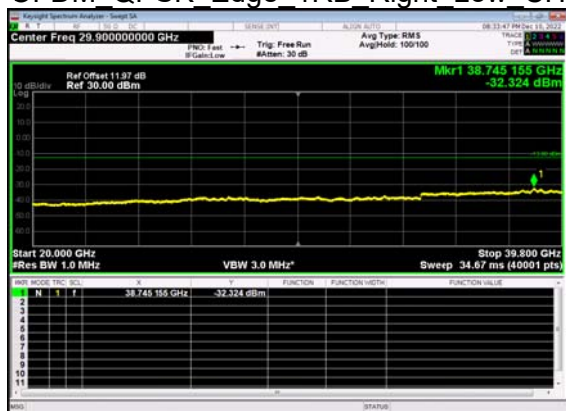
N77(50M)_DFT-s- OFDM QPSK Edge 1RB Right Low CH
