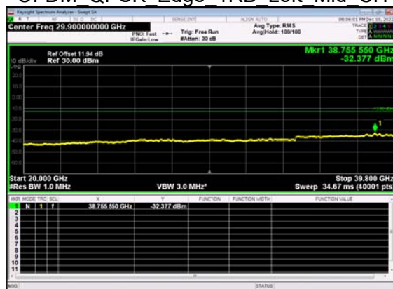
N77(40M)_DFT-s- OFDM QPSK Edge 1RB Left Mid CH
