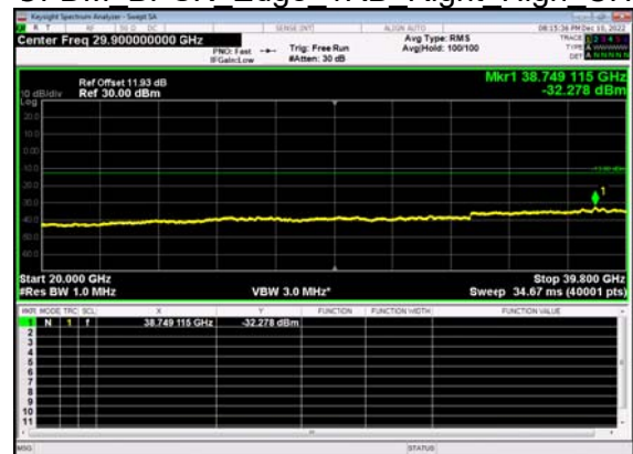
N77(40M)_DFT-s- OFDM BPSK Edge 1RB Right High CH
