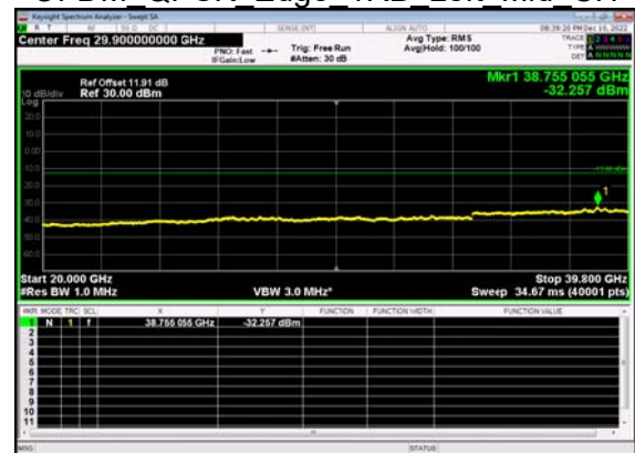
N77(50M)_DFT-s- OFDM QPSK Edge 1RB Left Mid CH
