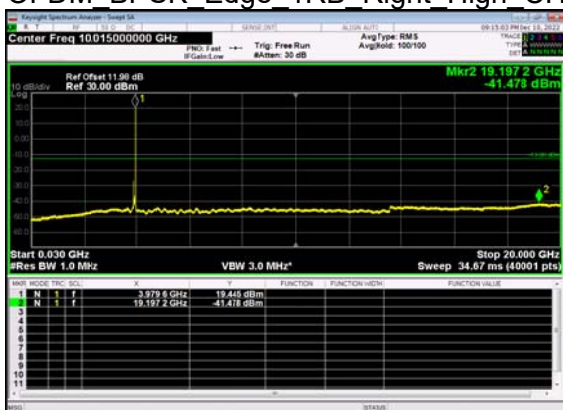
N77(60M)_DFT-s- OFDM BPSK Edge 1RB Right High CH
