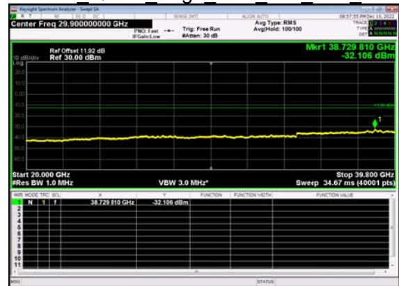
N77(60M)_DFT-s- OFDM QPSK Edge 1RB Left Low CH
