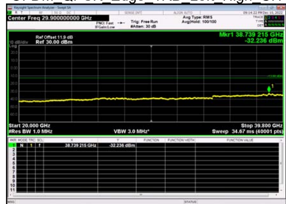
N77(60M)_DFT-s- OFDM QPSK Edge 1RB Left High CH
