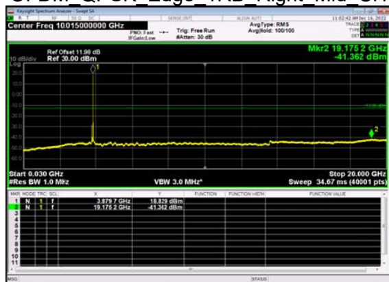
N77(80M)_DFT-s- OFDM QPSK Edge 1RB Right Mid CH
