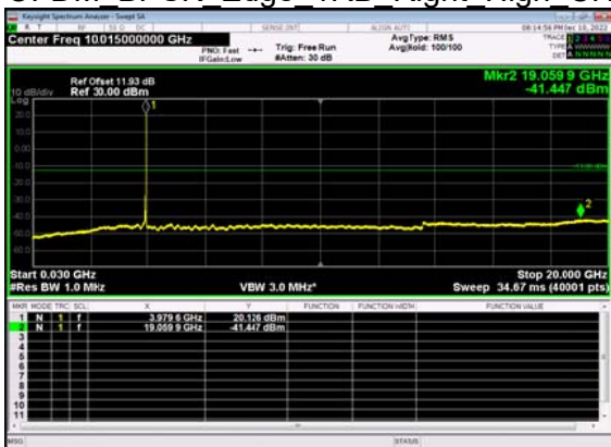
N77(40M)_DFT-s- OFDM BPSK Edge 1RB Right High CH
