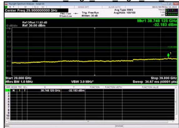
N77(50M)_DFT-s- OFDM QPSK Edge 1RB Right Mid CH
