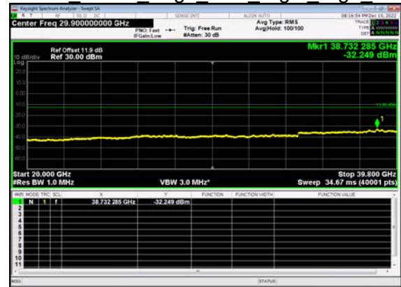
N77(40M)_DFT-s- OFDM QPSK Edge 1RB Right High CH
