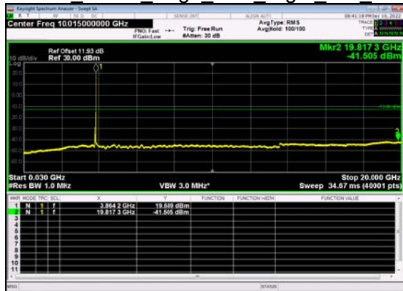
N77(50M)_DFT-s- OFDM QPSK Edge 1RB Right Mid CH
