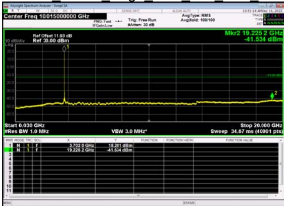
N77(80M)_DFT-s- OFDM QPSK Edge 1RB Left Low CH
