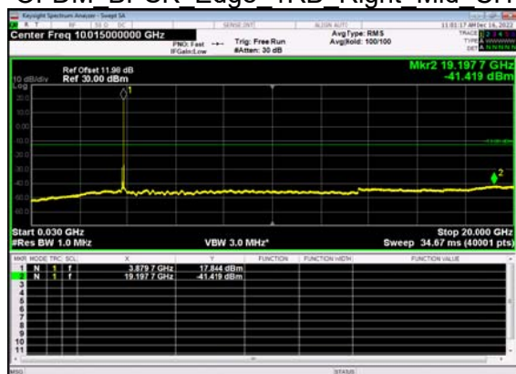
N77(80M)_DFT-s- OFDM BPSK Edge 1RB Right Mid CH
