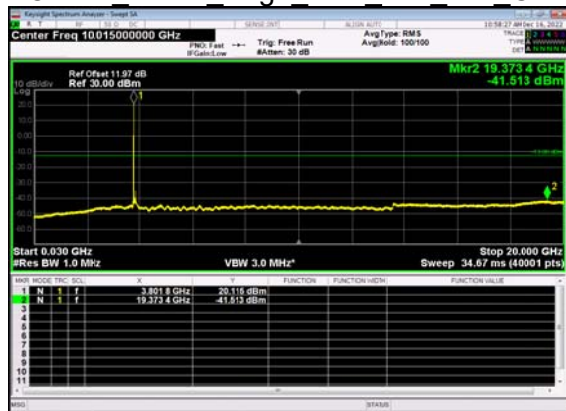
N77(80M)_DFT-s- OFDM BPSK Edge 1RB Left Mid CH
