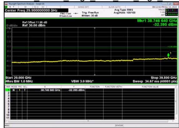
N77(40M)_DFT-s- OFDM BPSK Edge 1RB Left High CH
