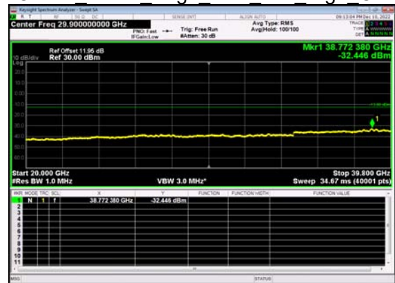
N77(60M)_DFT-s- OFDM BPSK Edge 1RB Left High CH
