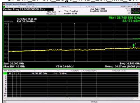
N77(40M)_DFT-s- OFDM BPSK Edge 1RB Left Mid CH
