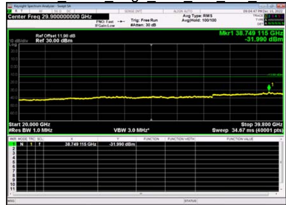
N77(60M)_DFT-s- OFDM BPSK Edge 1RB Left Mid CH
