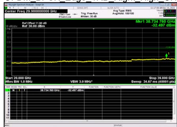
N77(80M)_DFT-s- OFDM BPSK Edge 1RB Right High CH
