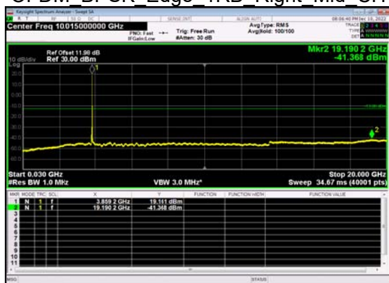
N77(40M)_DFT-s- OFDM BPSK Edge 1RB Right Mid CH
