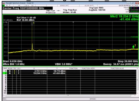
N77(60M)_DFT-s- OFDM BPSK Edge 1RB Left Low CH
