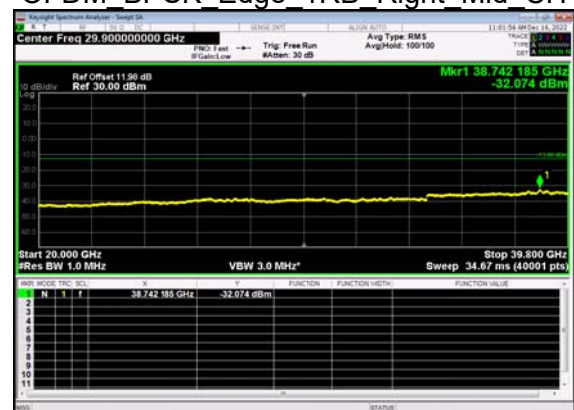
N77(80M)_DFT-s- OFDM BPSK Edge 1RB Right Mid CH
