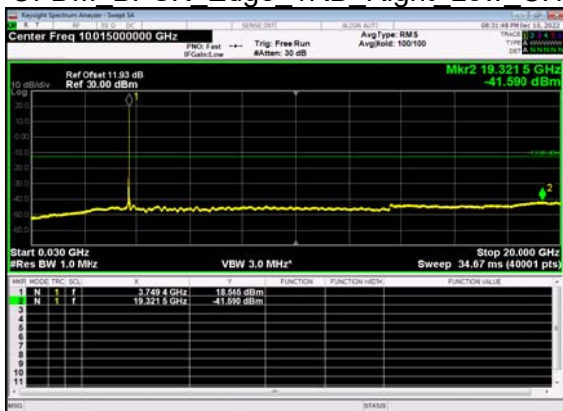
N77(50M)_DFT-s- OFDM BPSK Edge 1RB Right Low CH
