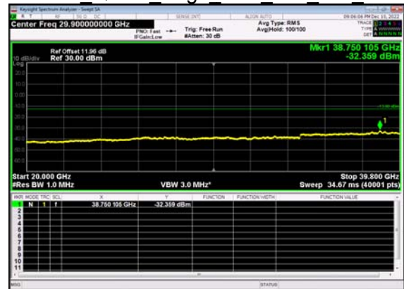
N77(60M)_DFT-s- OFDM QPSK Edge 1RB Left Mid CH
