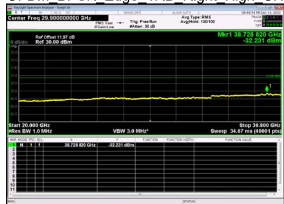
N77(50M)_DFT-s- OFDM BPSK Edge 1RB Right High CH
