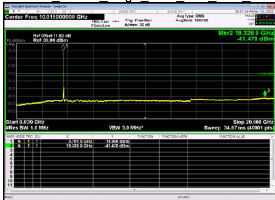
N77(60M)_DFT-s- OFDM QPSK Edge 1RB Left Low CH
