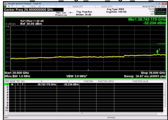
N77(40M)_DFT-s- OFDM QPSK Edge 1RB Right Mid CH
