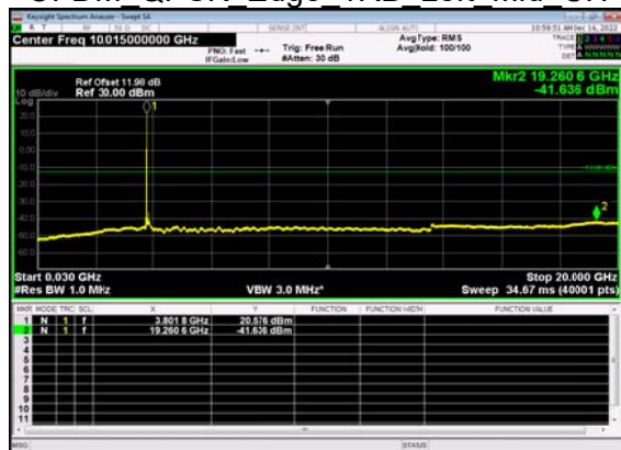
N77(80M)_DFT-s- OFDM QPSK Edge 1RB Left Mid CH
