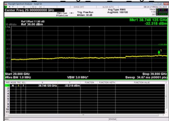
N77(40M)_DFT-s- OFDM QPSK Edge 1RB Left High CH
