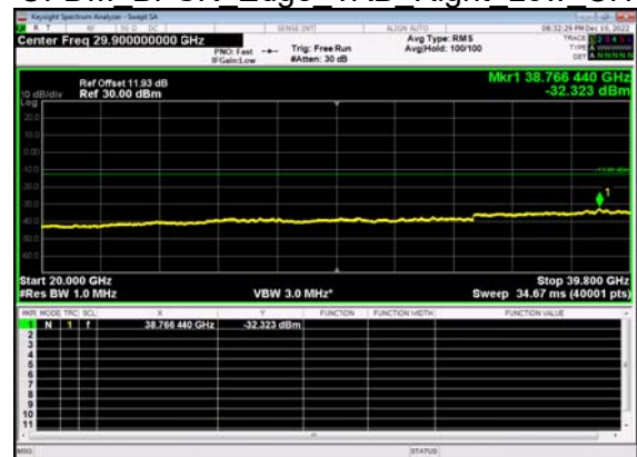
N77(50M)_DFT-s- OFDM BPSK Edge 1RB Right Low CH
