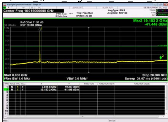
N77(50M)_DFT-s- OFDM QPSK Edge 1RB Left Mid CH
