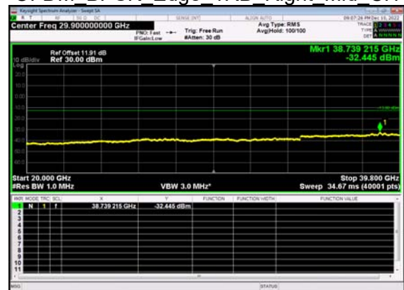
N77(60M)_DFT-s- OFDM BPSK Edge 1RB Right Mid CH
