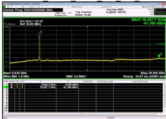
N77(50M)_DFT-s- OFDM BPSK Outer Full Mid CH
