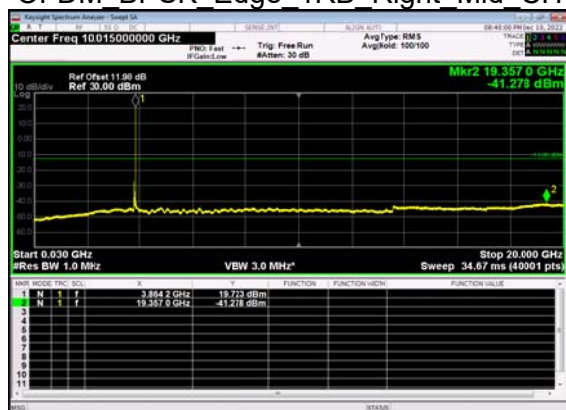
N77(50M)_DFT-s- OFDM BPSK Edge 1RB Right Mid CH
