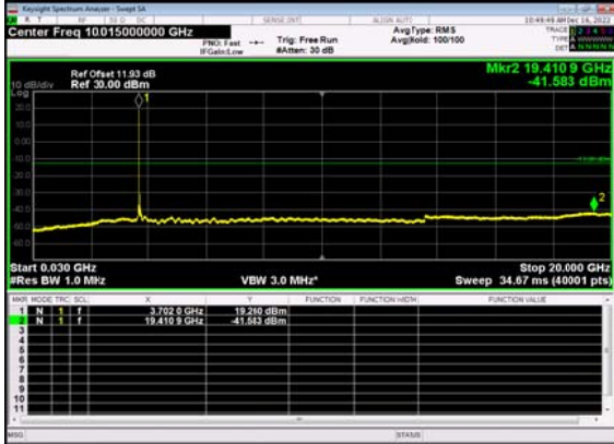
N77(80M)_DFT-s- OFDM BPSK Edge 1RB Left Low CH
