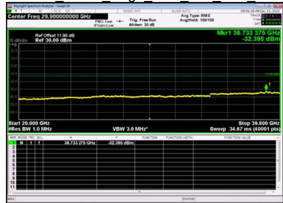
N77(60M)_DFT-s- OFDM BPSK Edge 1RB Left Low CH
