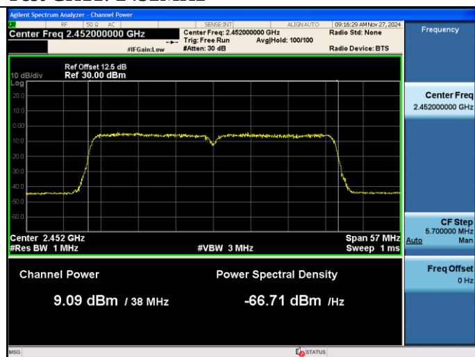
Test CH11: 2452MHz
