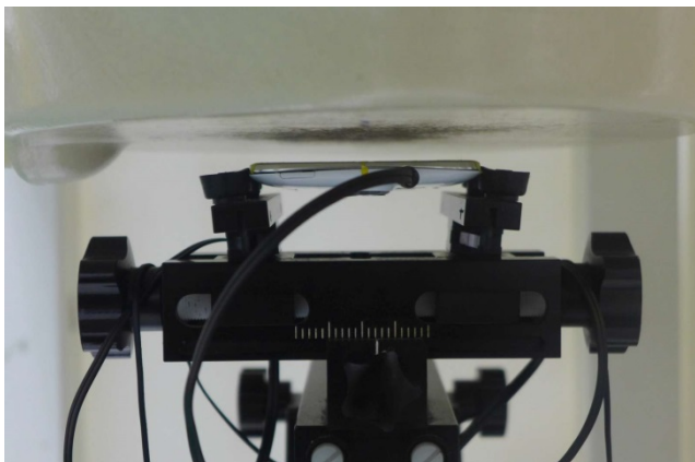
Front of the DUT with Phantom 1 cm Gap (with / headset)
