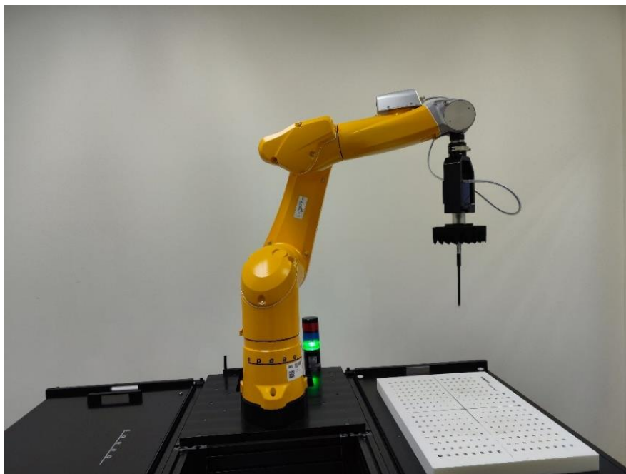
Fig.2 Photograph of the mmWave measurement system
