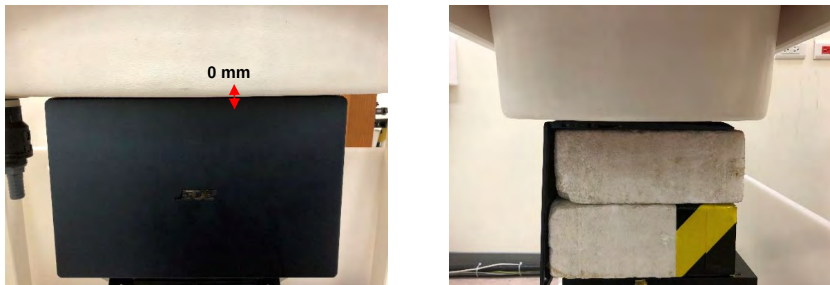
Fig.3 EUT Bottom side to flat phantom
