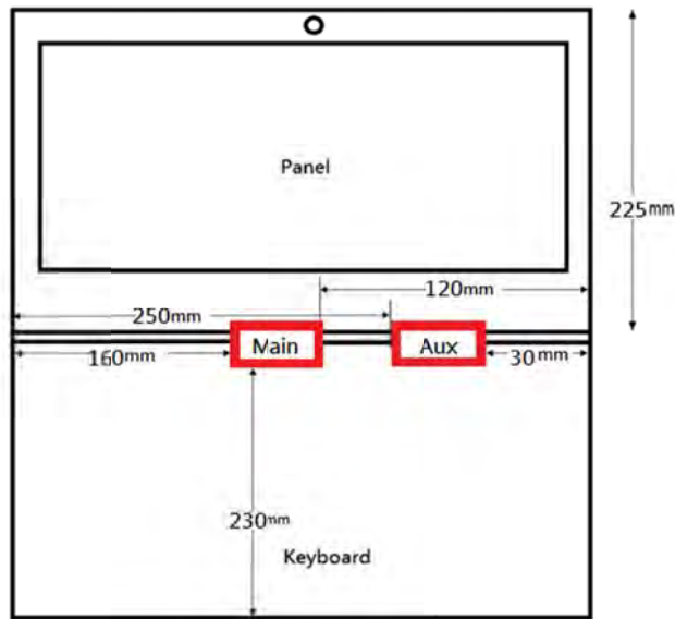
Fig.6 Antenna position of EUT (Front view)
