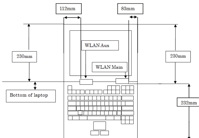
Fig.6 Antenna position of EUT (Front view)
