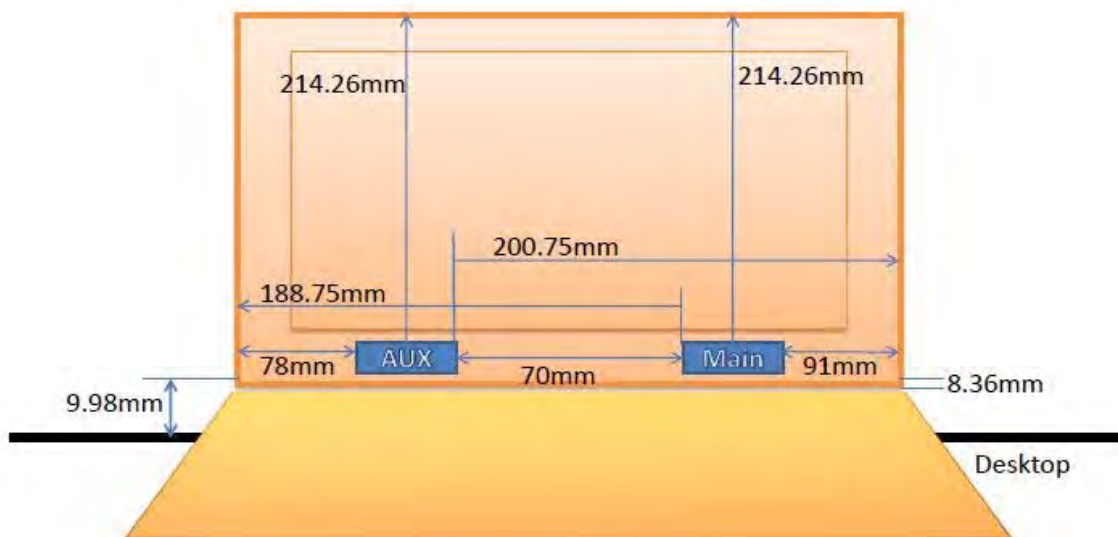
Fig.6 Antenna position of EUT (Front view)
