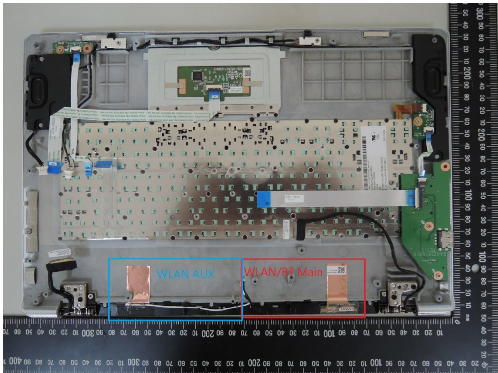
BT/WLAN Antenna Location
