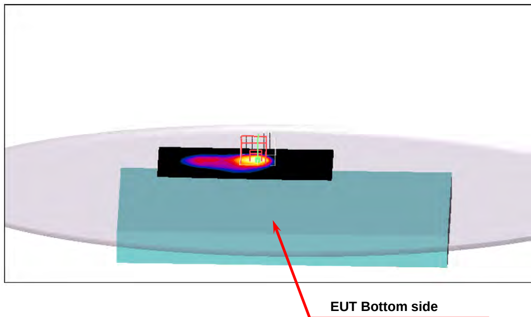
Figure 1. Body SAR Test Setup (Flat Section) Host: LCD Open 90° Bottom Close Body
