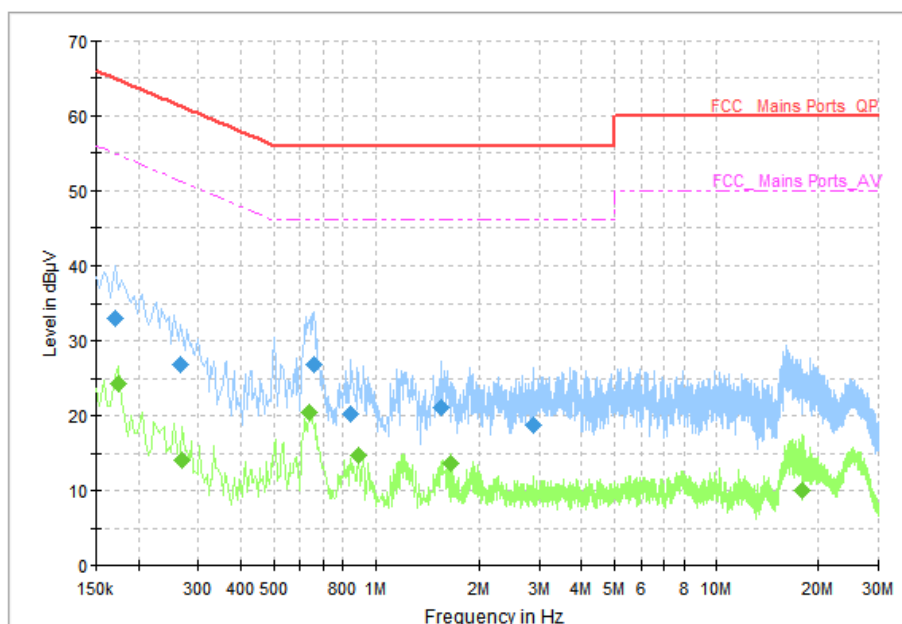
Figure A-6 Conducted Emission (Idle)-AE4,AE5
