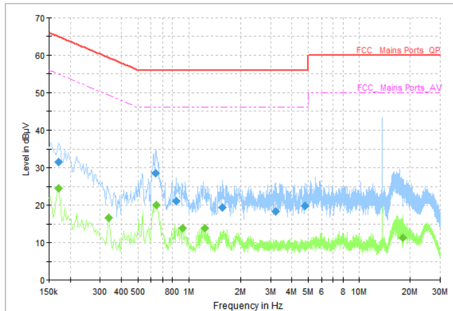
Figure A-5 Conducted Emission (Traffic)-AE4,AE5
