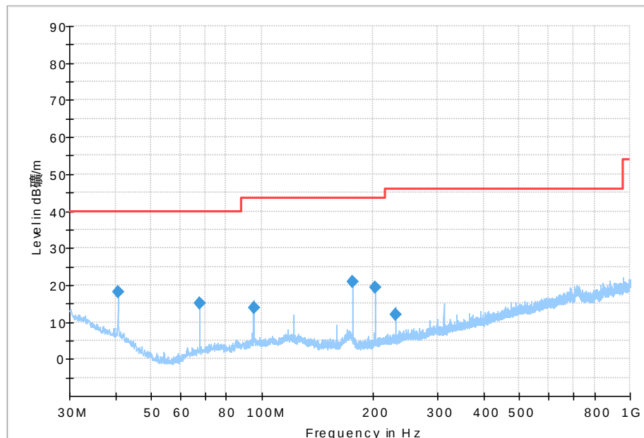
Figure A-3 Transmit State (30M-1G)
