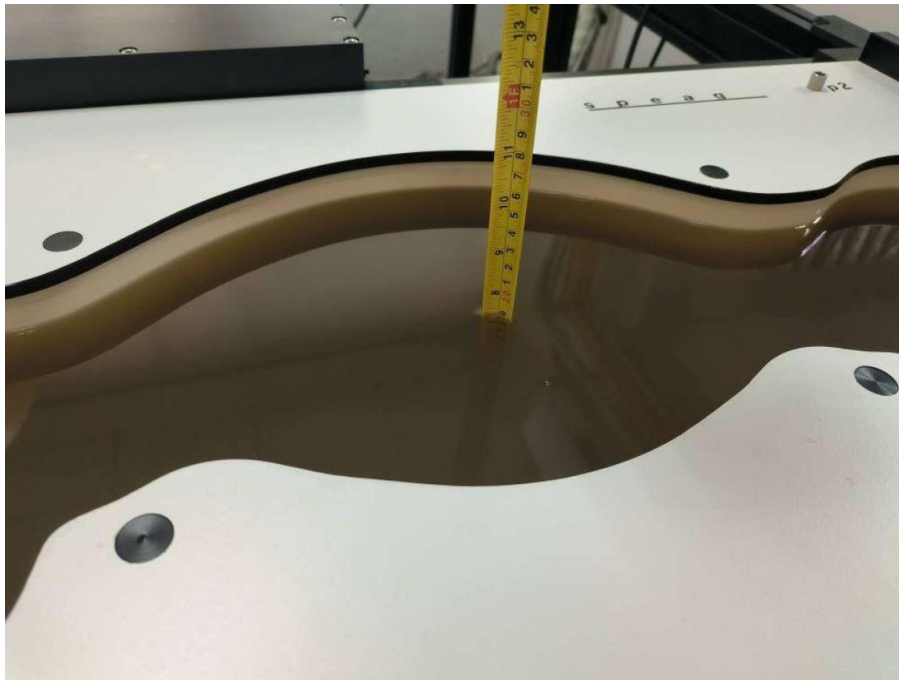
Picture 7.1 Liquid depth in the Flat Phantom (2GHz - 8GHz)
