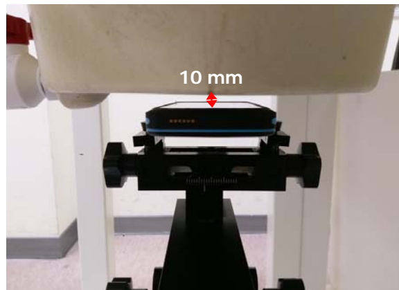
Fig.12 EUT Front side to flat phantom
