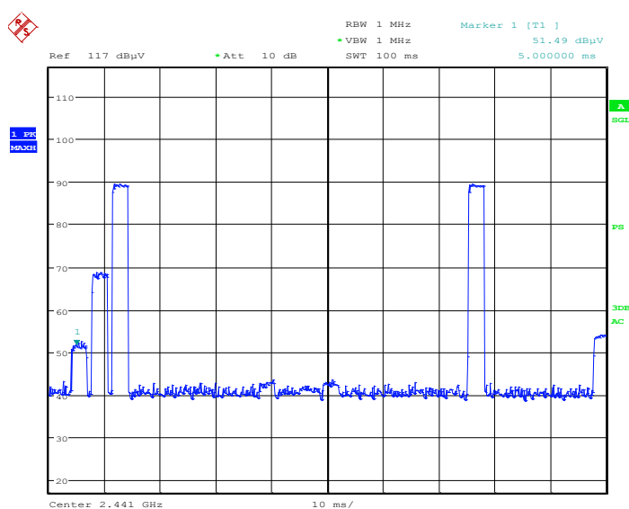
2DH5 on time/100ms (Count Pulses) Plot on Channel 39
