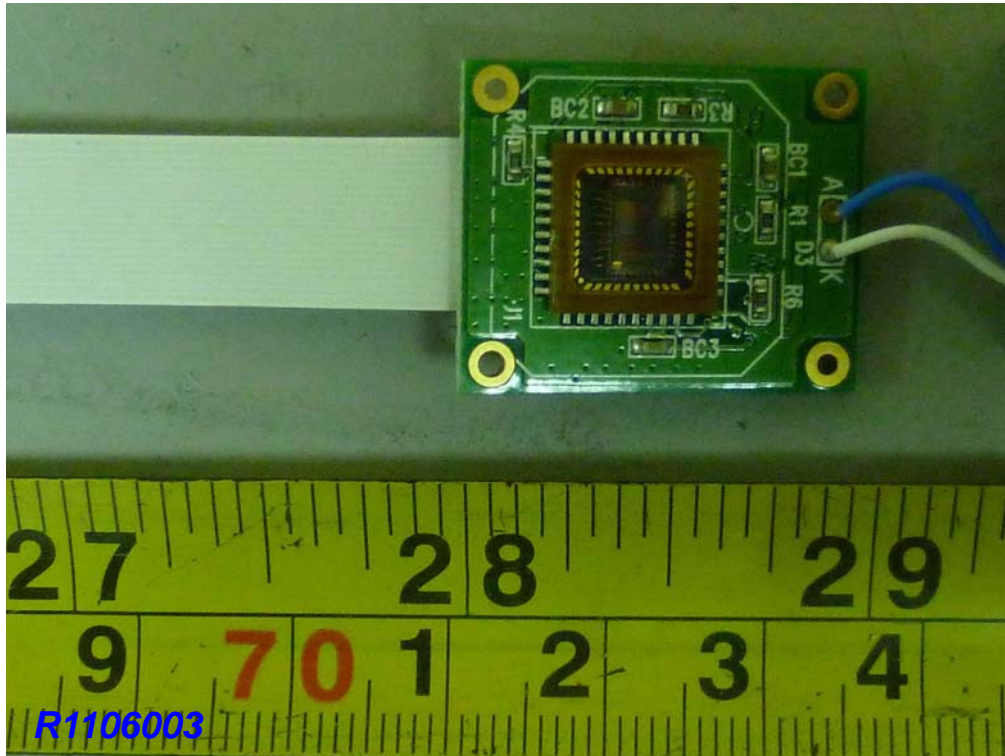
Model Name: MT650-AQUEAG FingerPrint board (SFM3020)
