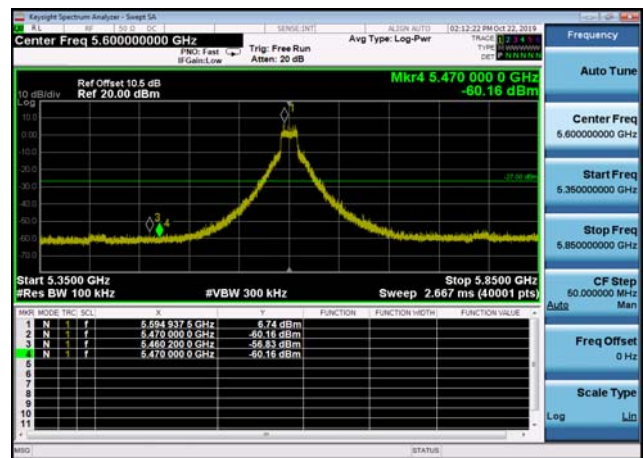
U-NII-2c ,Plot 1,Band Edge-802.11a(20 MHz),5600MHz
