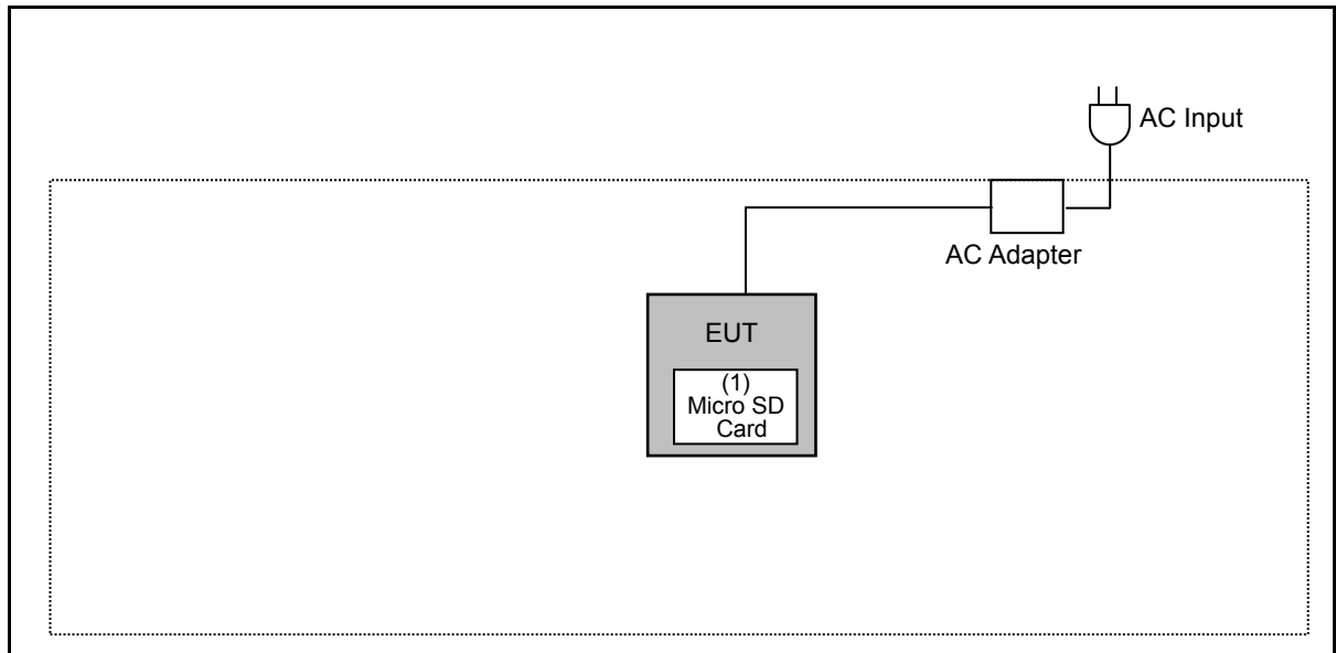
Radiated Emissions
