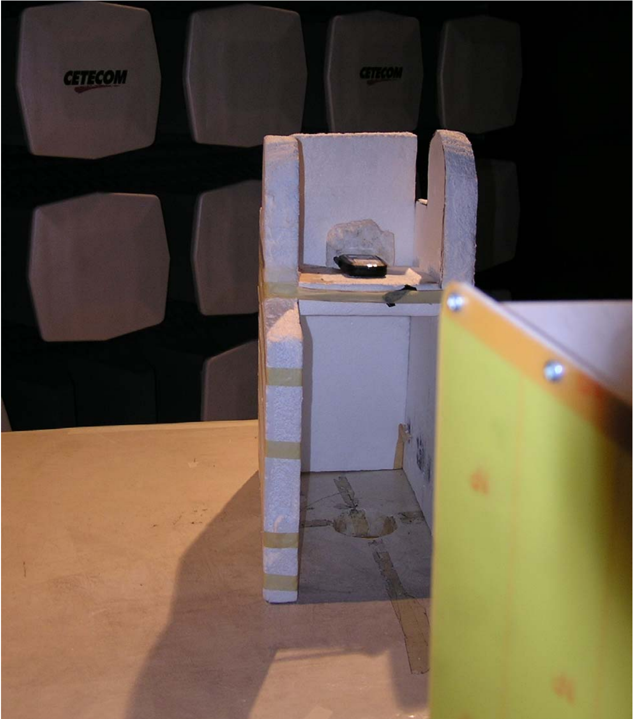
EIRP - Measurements
