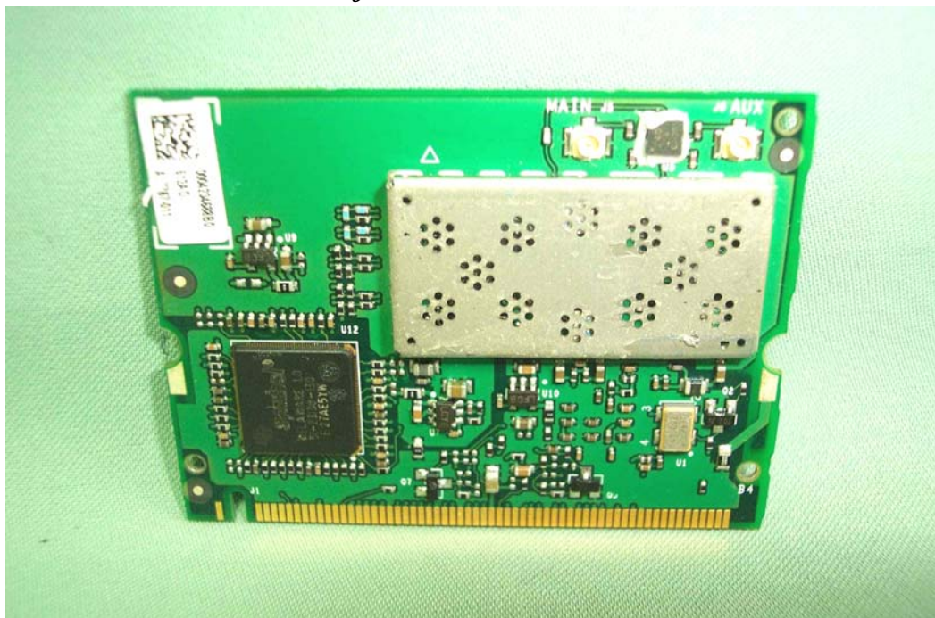
Front of Wireless LAN Module-1
