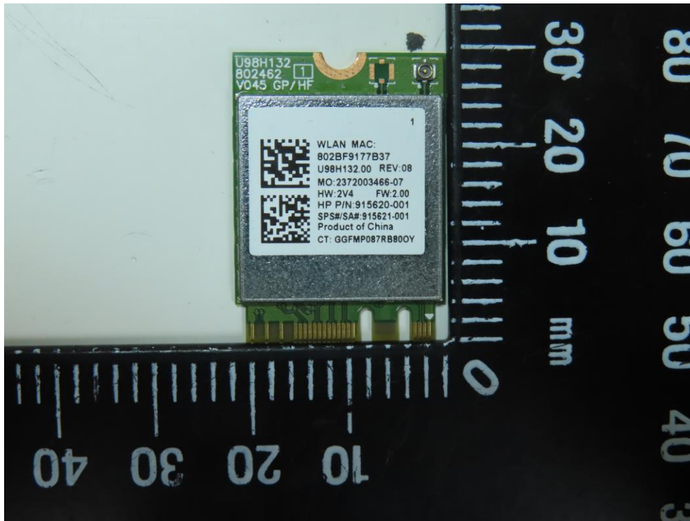
WLAN / BT Module -1 (Model No. :RTL8821CE)
