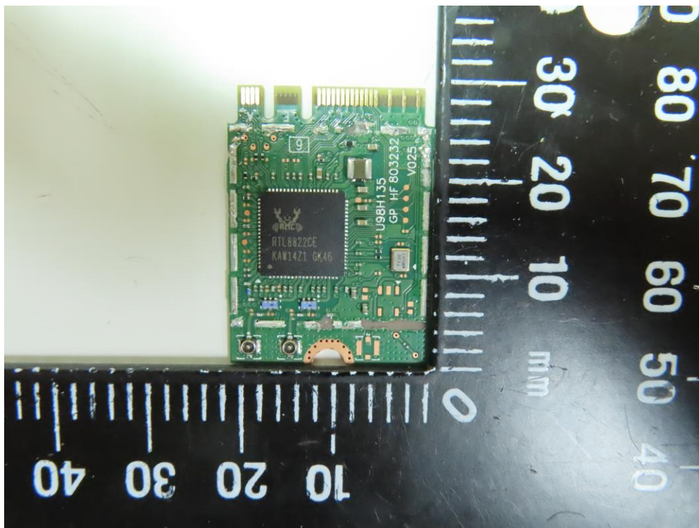
WLAN / BT Module -3 (Model No. : RTL8822CE)
