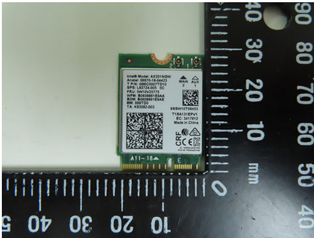
WLAN / BT Module -2 (Model No.: AX201NGW)
