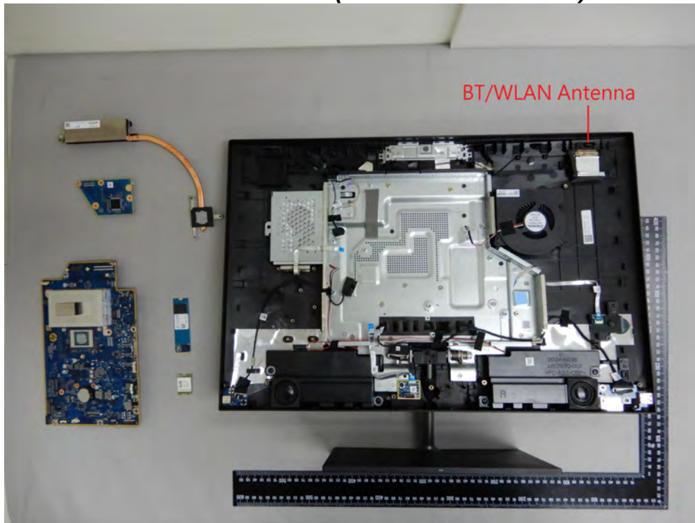
WLAN / BT Module -1 (Model No.:RTL8822CE)
