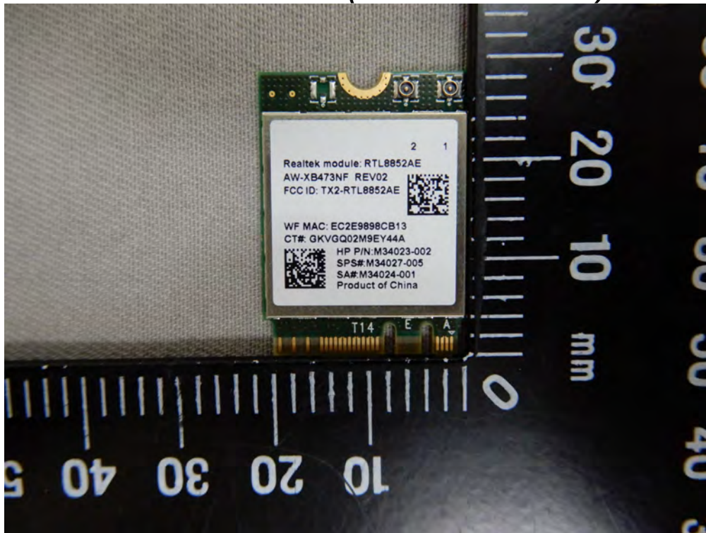
WLAN / BT Module -2 (Model No.:RTL8852AE)
