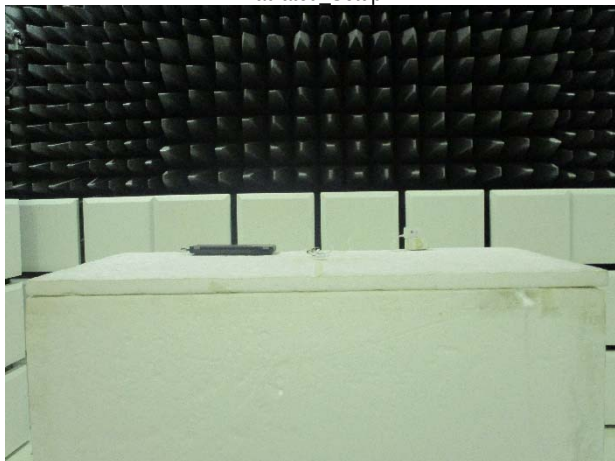
Radiated Setup
