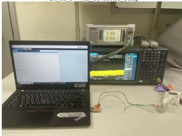
Part 15 247 LE Conducted Setup
