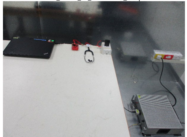
Part_15.247_LE_Conduction_Setup
